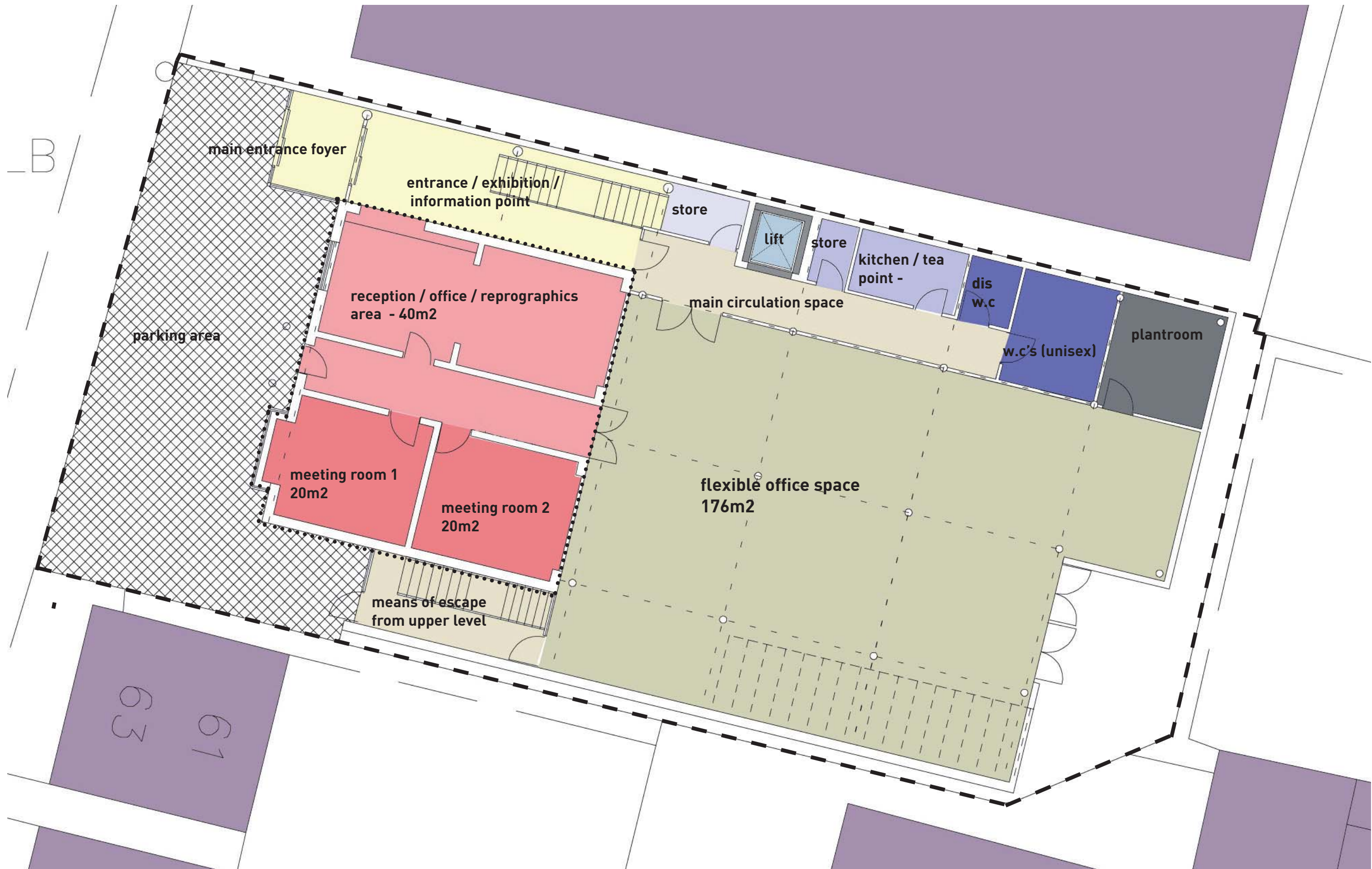
Development of 29 Church Street, Slough - Proposed Ground Floor Plan - Phase 2
